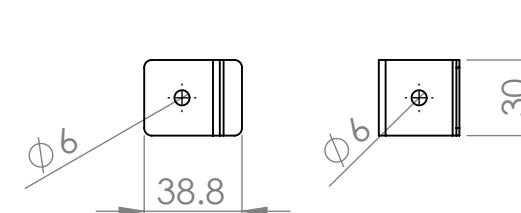
FIXING LUGS SCALE:1:3@A3
