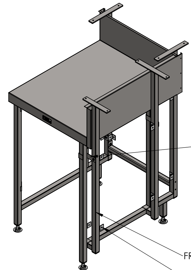
FRAME BRACKET
