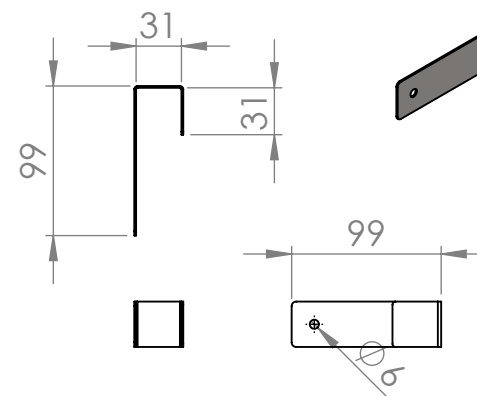
FRAME BRACKET SCALE:1:5@A3
