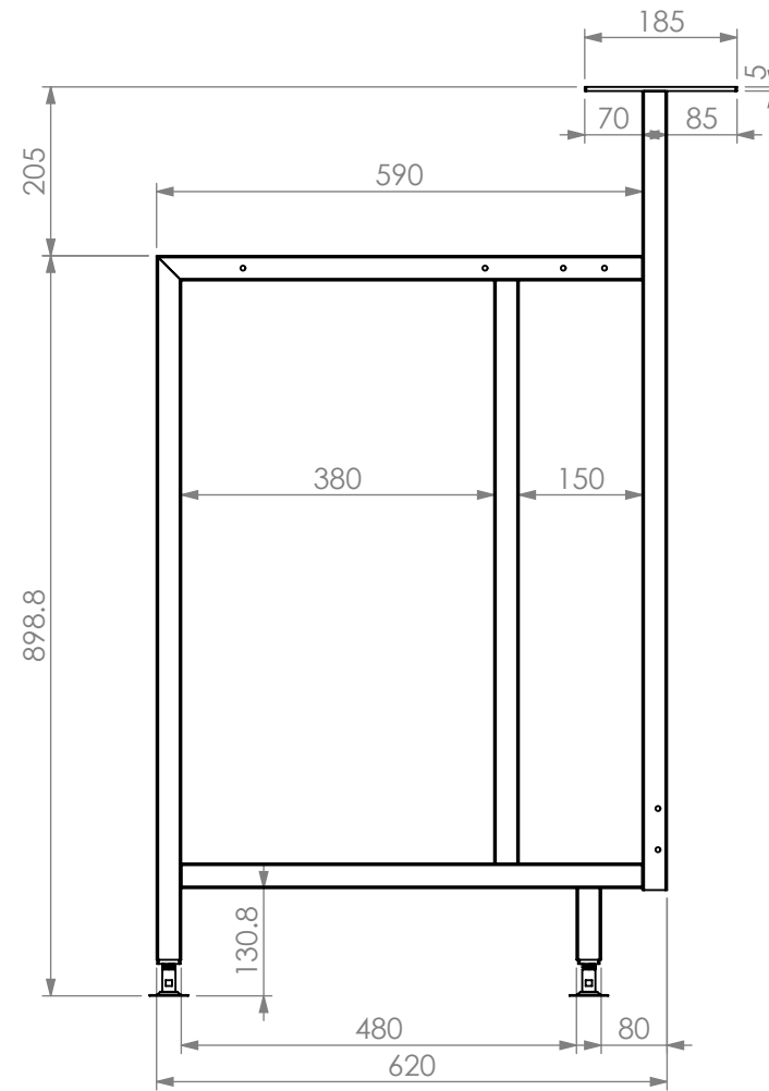
SIDE ELEVATION
