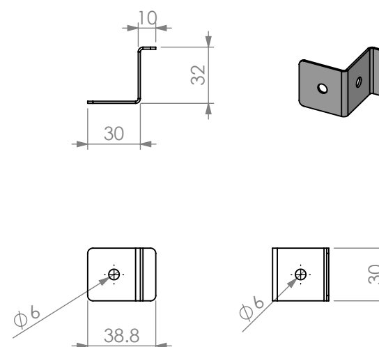
FIXING LUGS SCALE:1:3@A3
