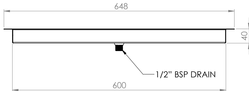
FRONT ELEVATION
