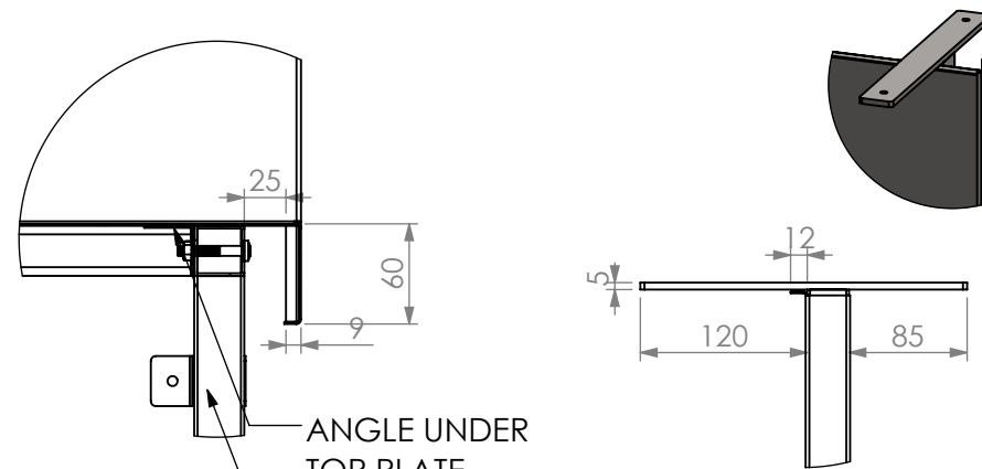
DETAIL A
