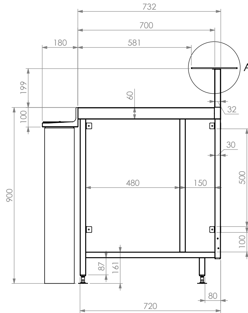
SIDE ELEVATION
