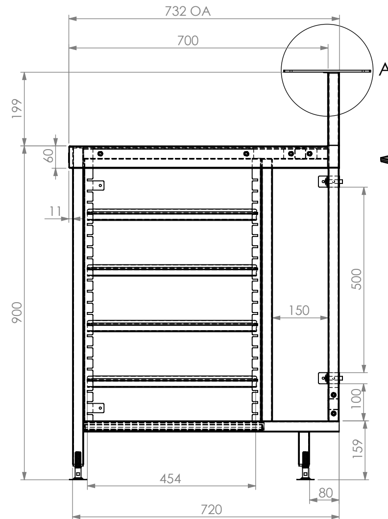
SIDE ELEVATION
