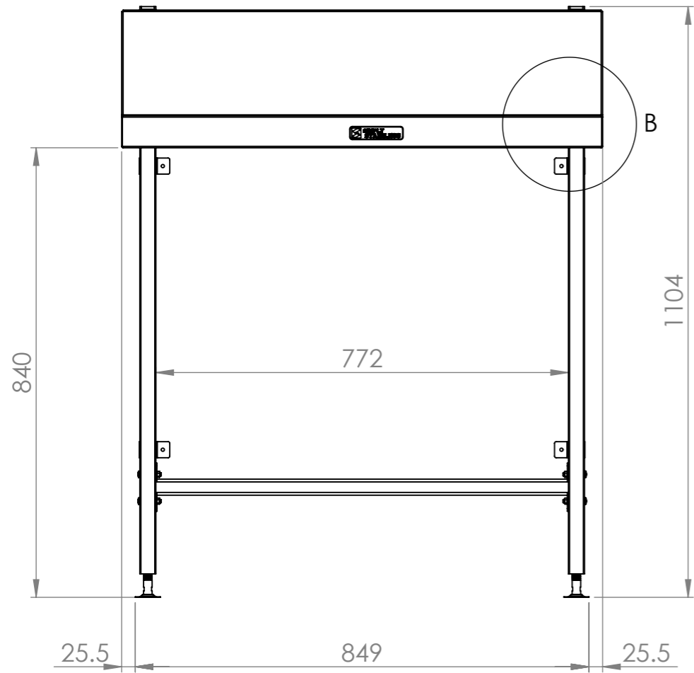
FRONT ELEVATION
