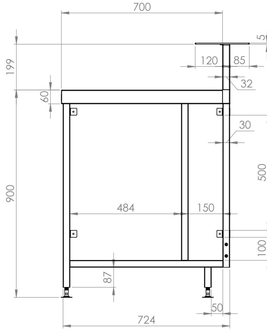
SIDE ELEVATION
