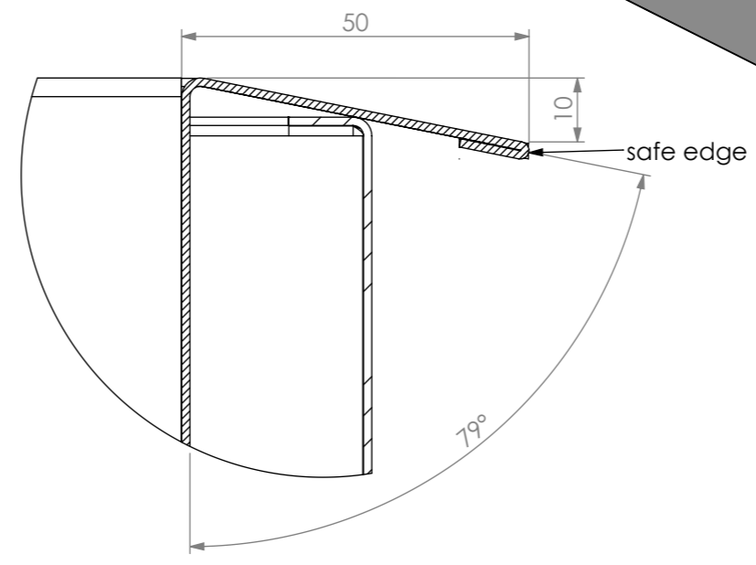
DETAIL P
