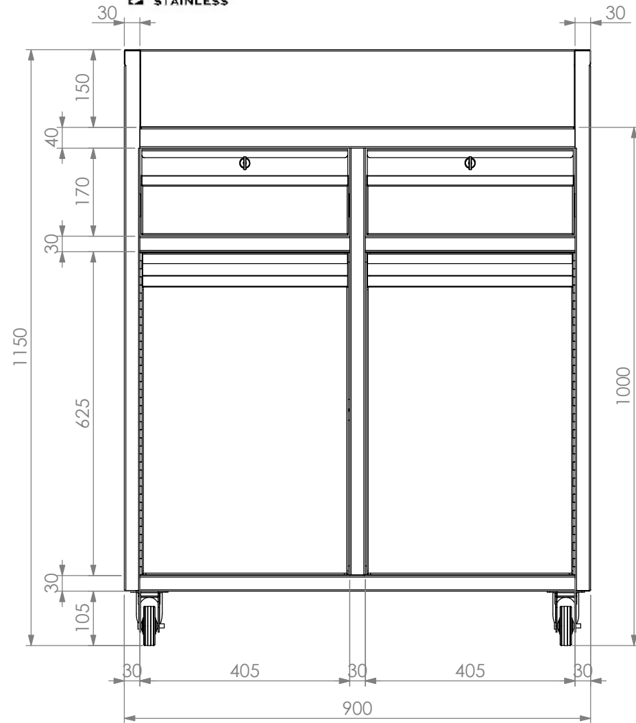
FRONT ELEVATION
