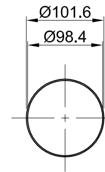
BOLLARD DETAIL SECTION/PLAN
