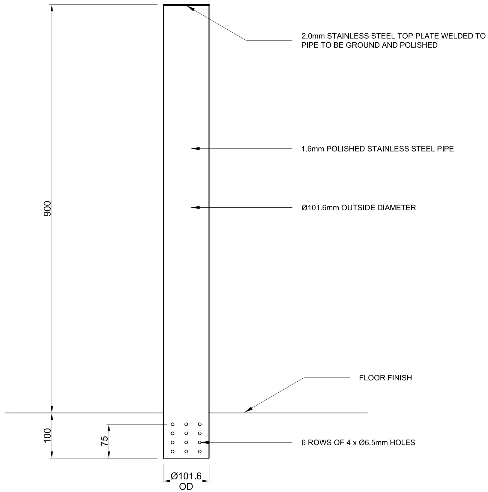
BOLLARD DETAIL SECTION THROUGH
