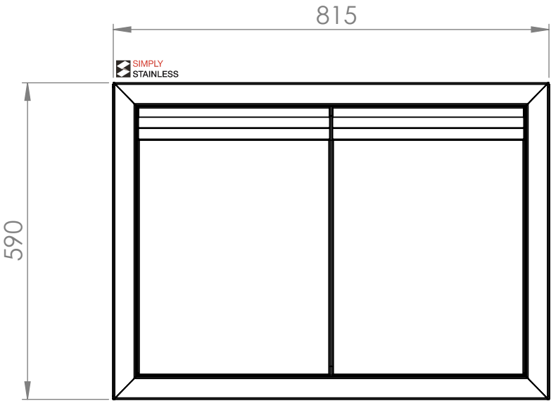
FRONT ELEVATION
