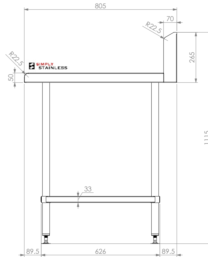
SIDE ELEVATION
