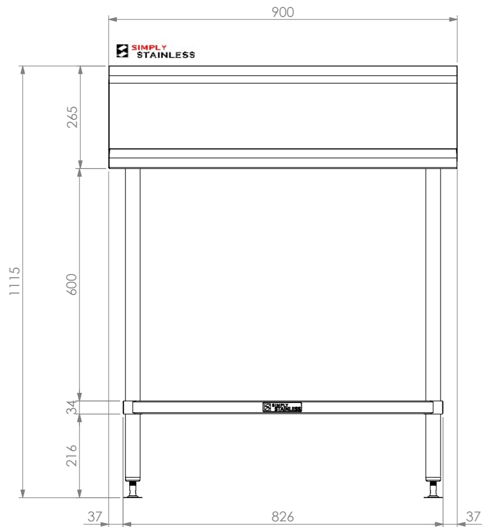
FRONT ELEVATION
