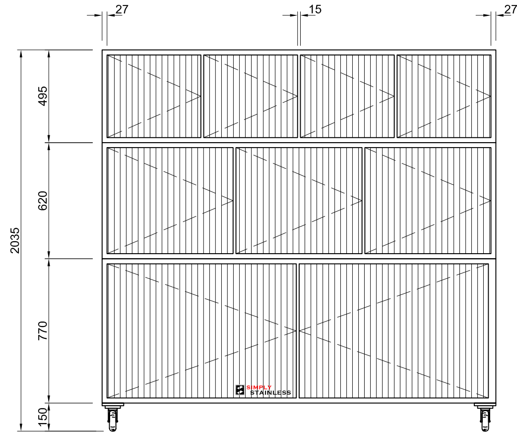
FRONT ELEVATION
