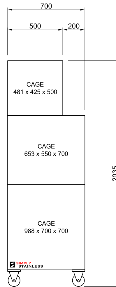
SIDE ELEVATION
