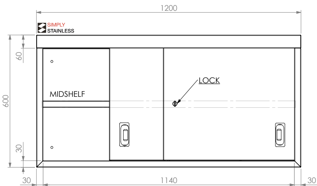
FRONT ELEVATION
