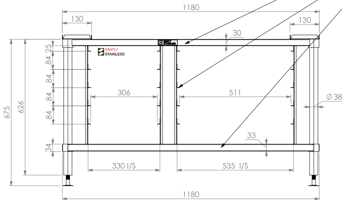
FRONT ELEVATION
