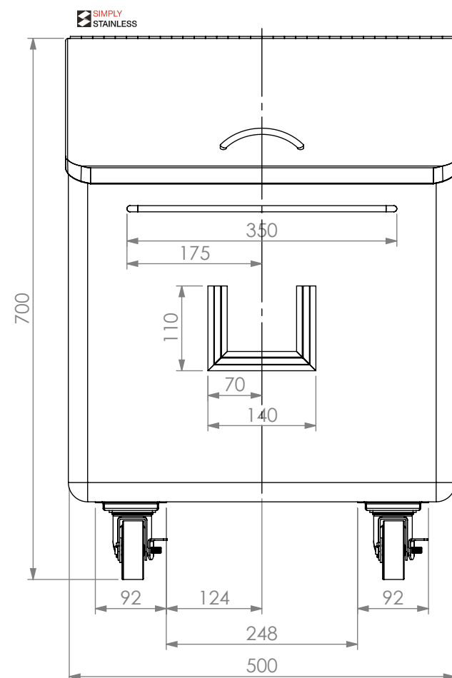
FRONT ELEVATION
