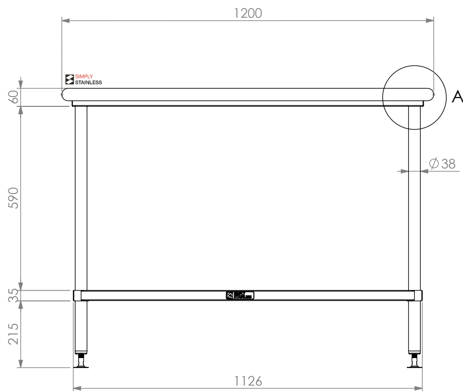
FRONT ELEVATION
