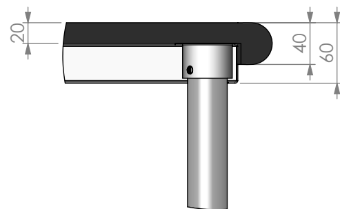
DETAIL A (GRANITE TOP DETAIL)
