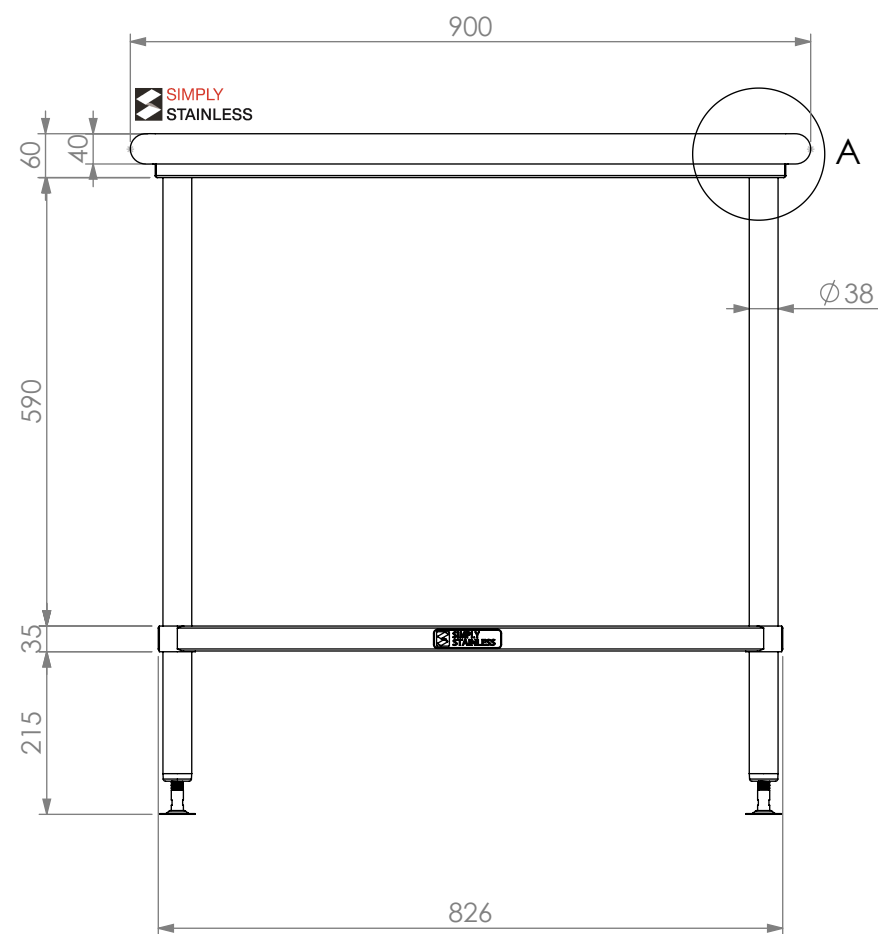
FRONT ELEVATION
