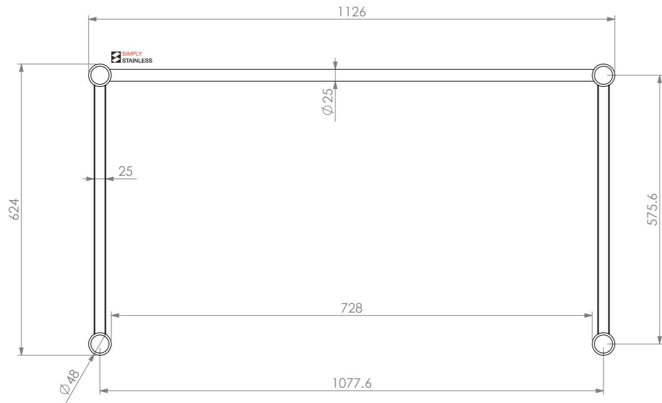
PLAN
