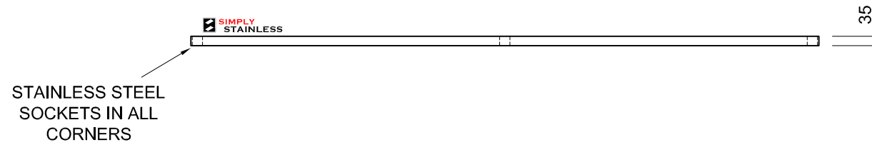
FRONT ELEVATION
