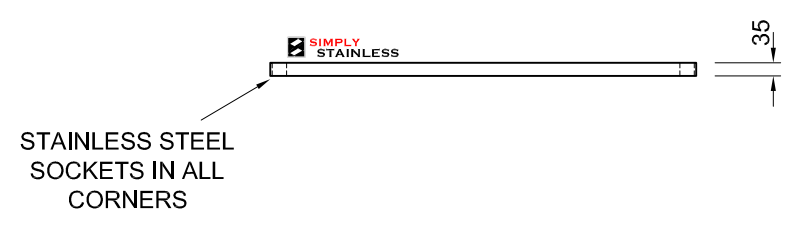
FRONT ELEVATION
