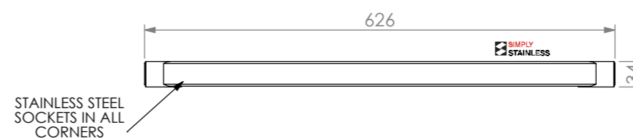
SIDE ELEVATION
