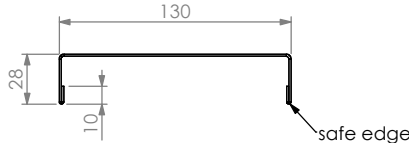
REINFORCING CHANNEL DETAILS
