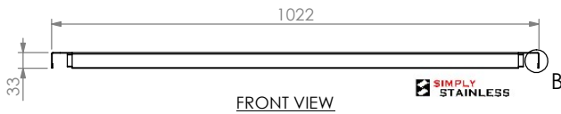
FRONT VIEW
