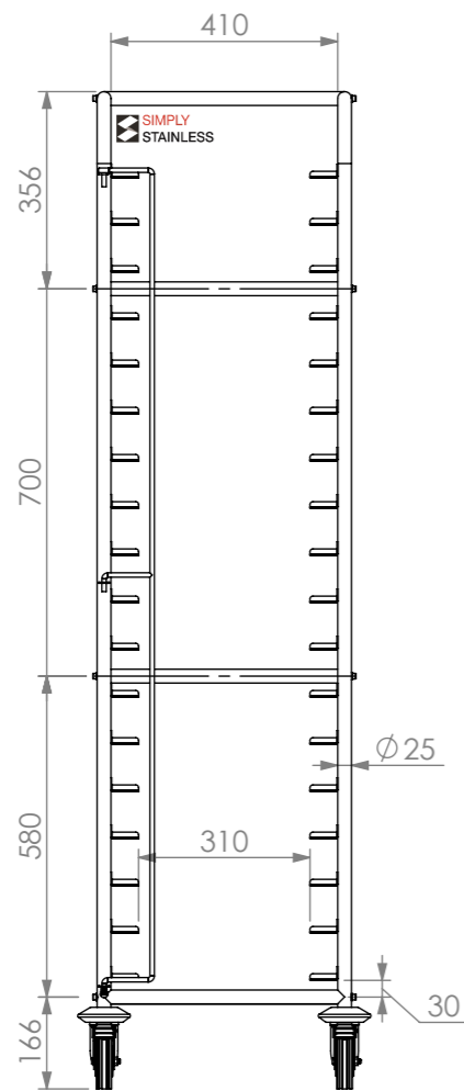
FRONT VIEW
