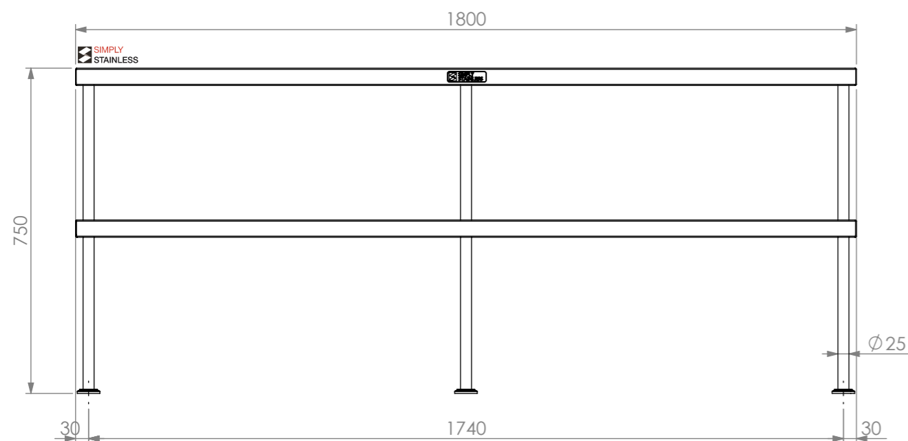
FRONT ELEVATION
