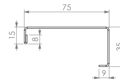
REINFORCING CHANNEL II DETAIL
