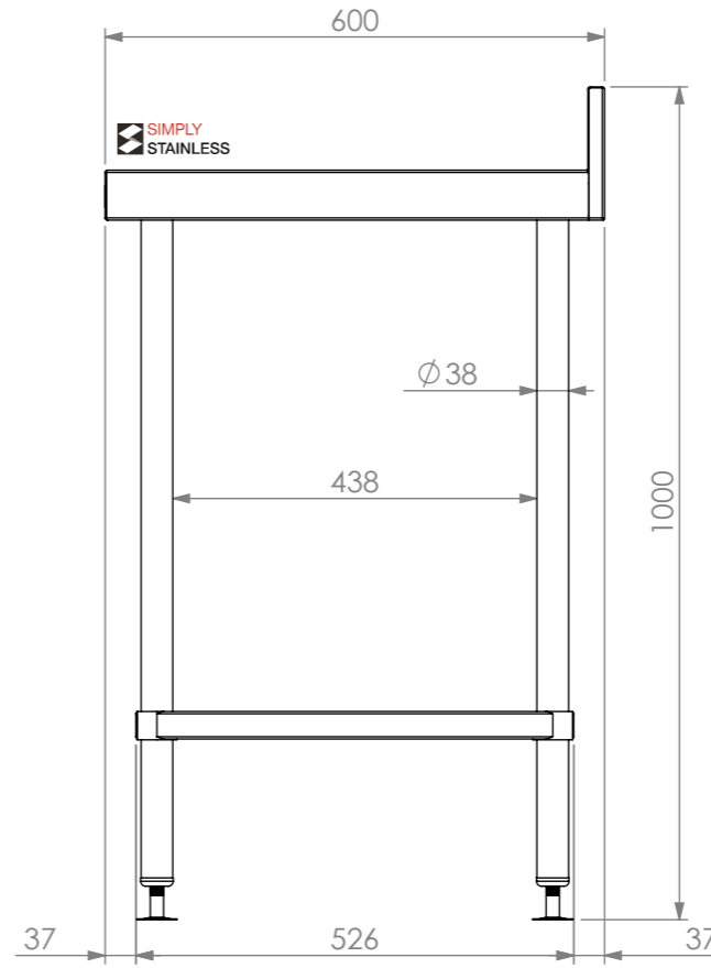
SIDE ELEVATION
