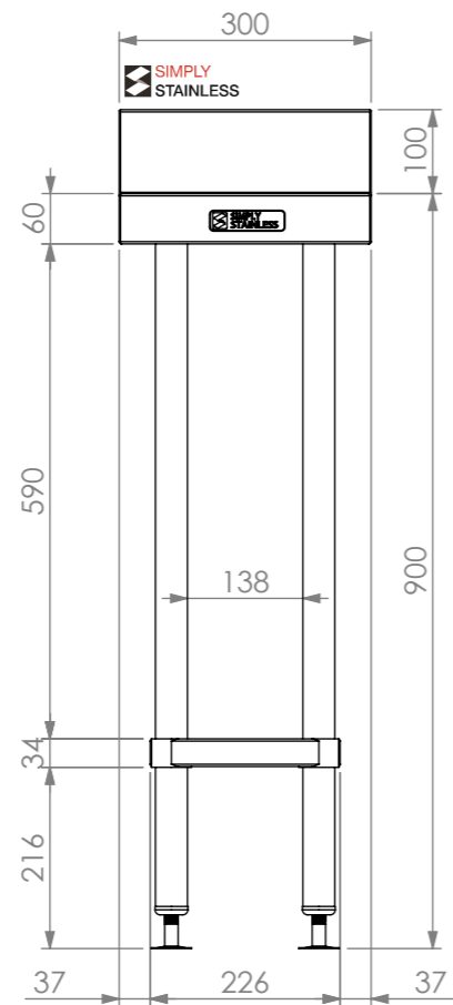
FRONT ELEVATION
