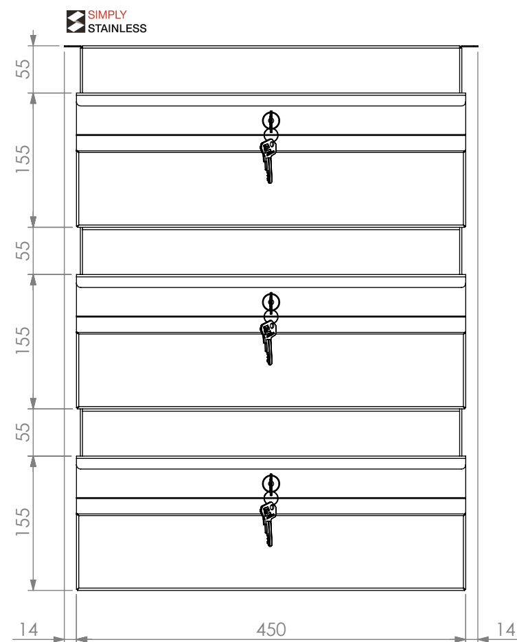
FRONT ELEVATION
