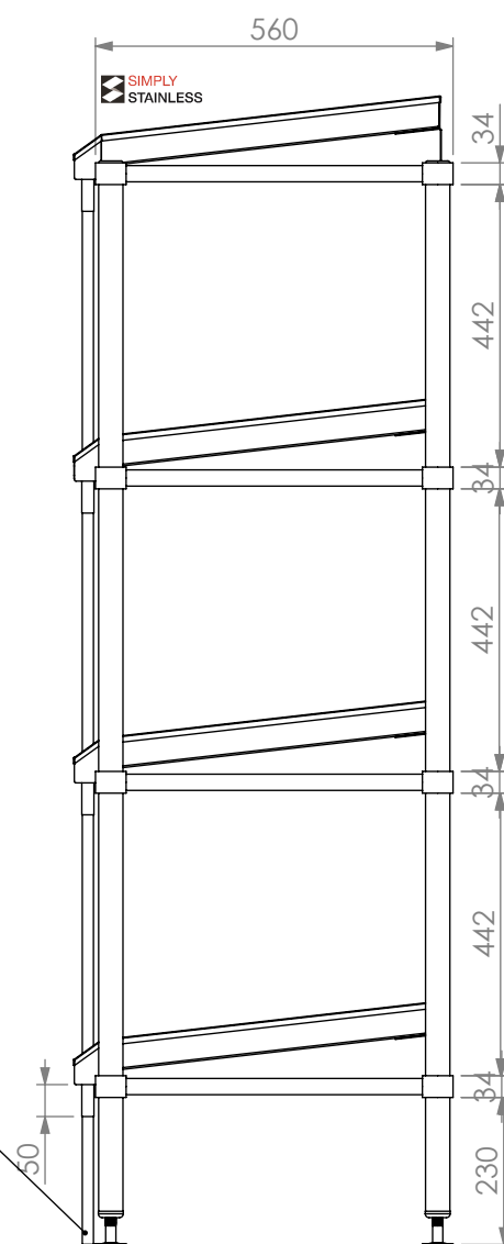
SIDE VIEW
