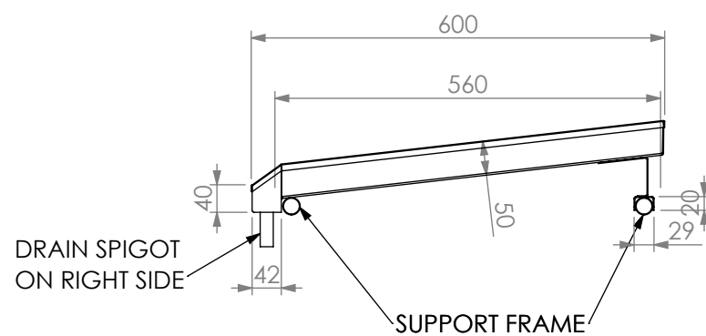
SHELF DETAIL
