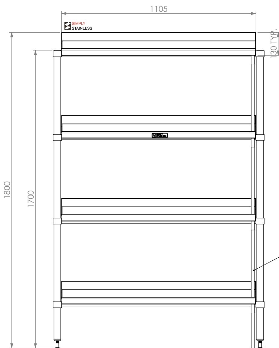
FRONT VIEW
