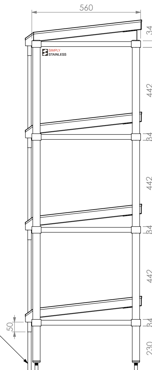
SIDE VIEW
