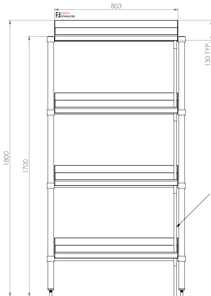
FRONT VIEW
