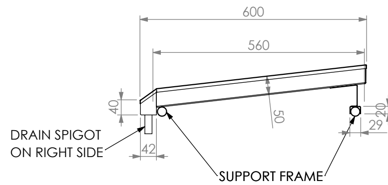
SHELF DETAIL
