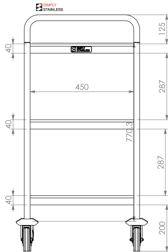
FRONT ELEVATION
