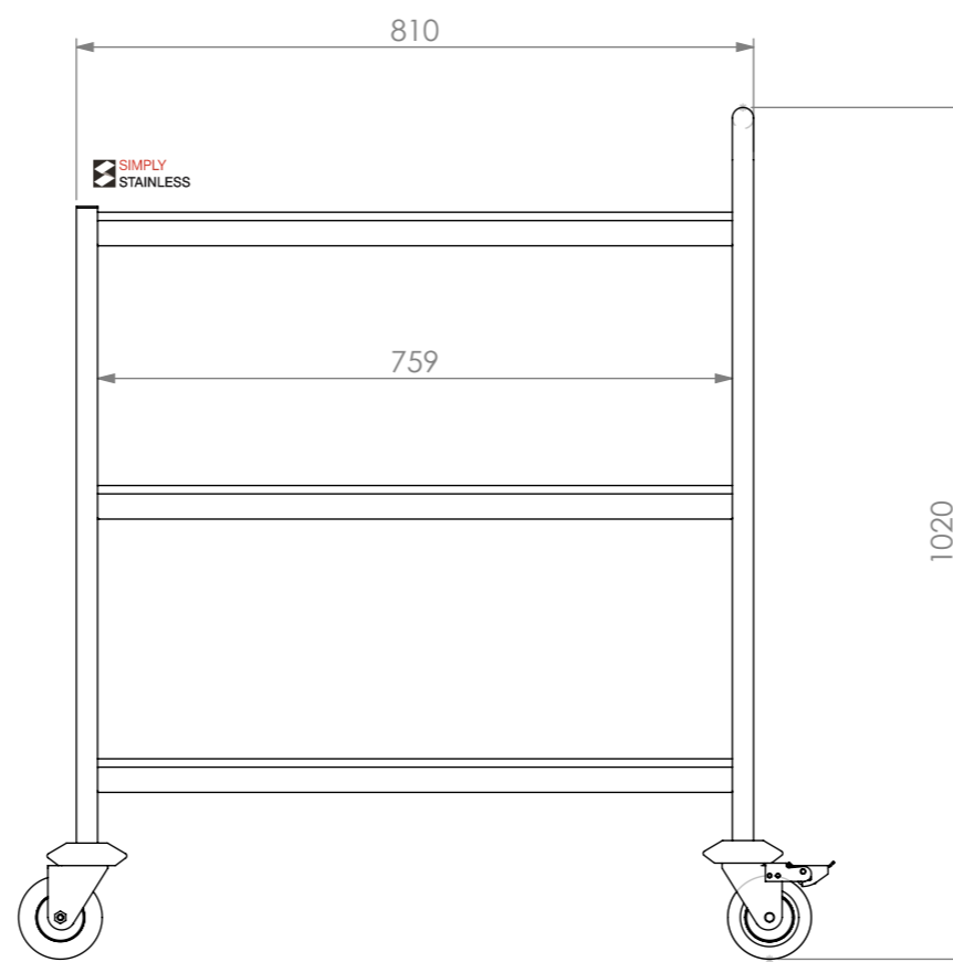
SIDE ELEVATION
