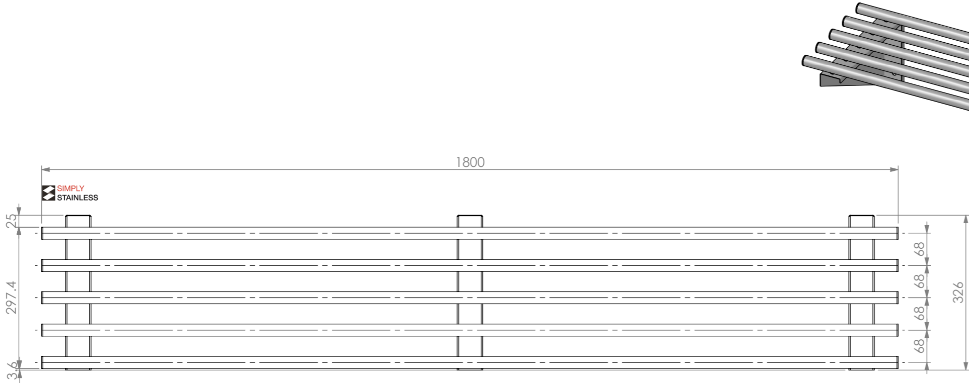
PLAN
