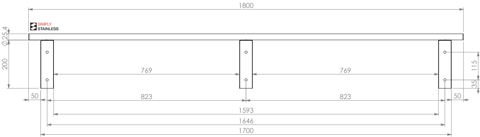
FRONT ELEVATION
