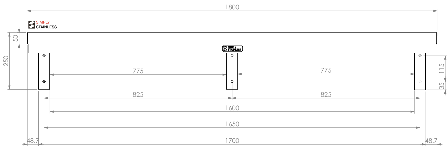
FRONT ELEVATION
