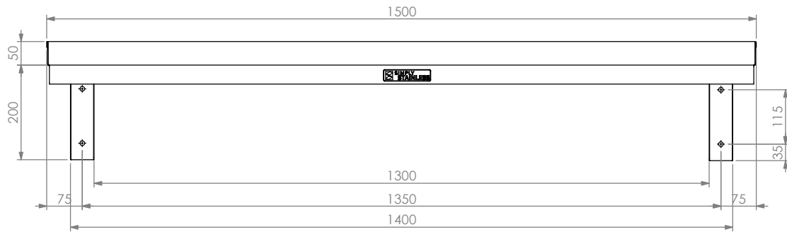
FRONT ELEVATION
