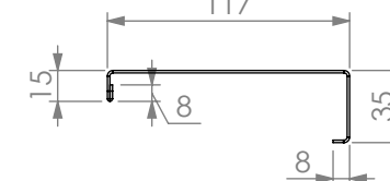
REINFORCING CHANNEL IV DETAIL
