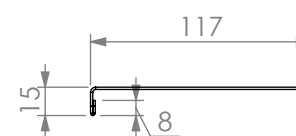
REINFORCING CHANNEL I DETAIL
