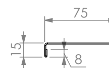
REINFORCING CHANNEL III DETAIL
