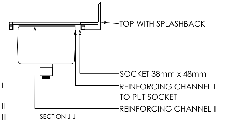
SECTION J-J
