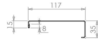
REINFORCING CHANNEL I DETAIL
