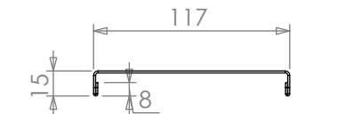
REINFORCING CHANNEL III DETAIL
