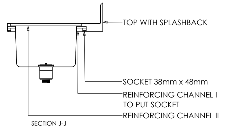
SECTION J-J
