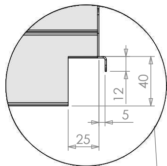
NOTCH DETAIL
