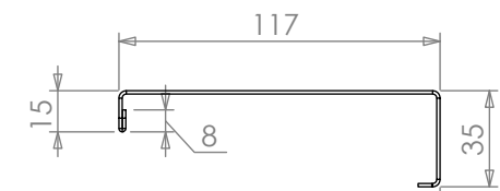
REINFORCING CHANNEL I DETAIL
