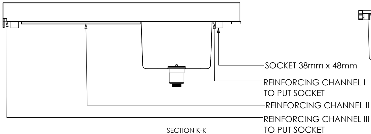
SECTION K-K
