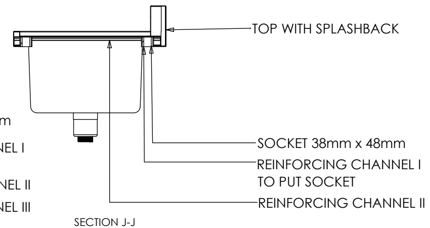
SECTION J-J
