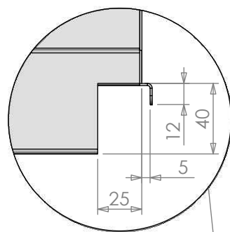
NOTCH DETAIL
