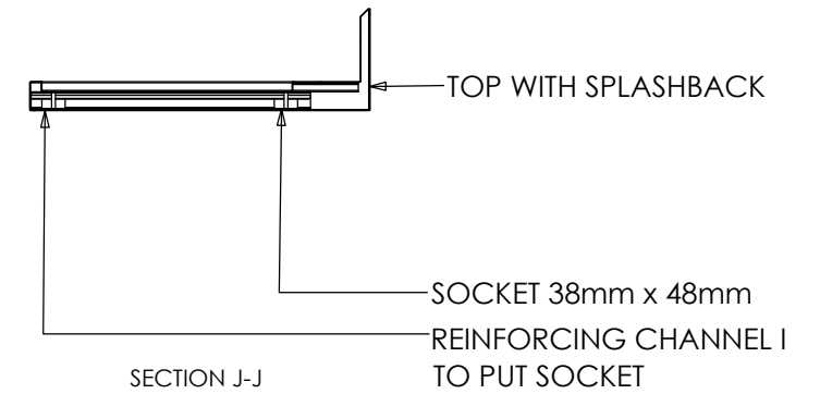
SECTION J-J
