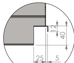
NOTCH DETAIL
