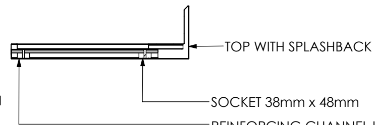
SECTION J-J
