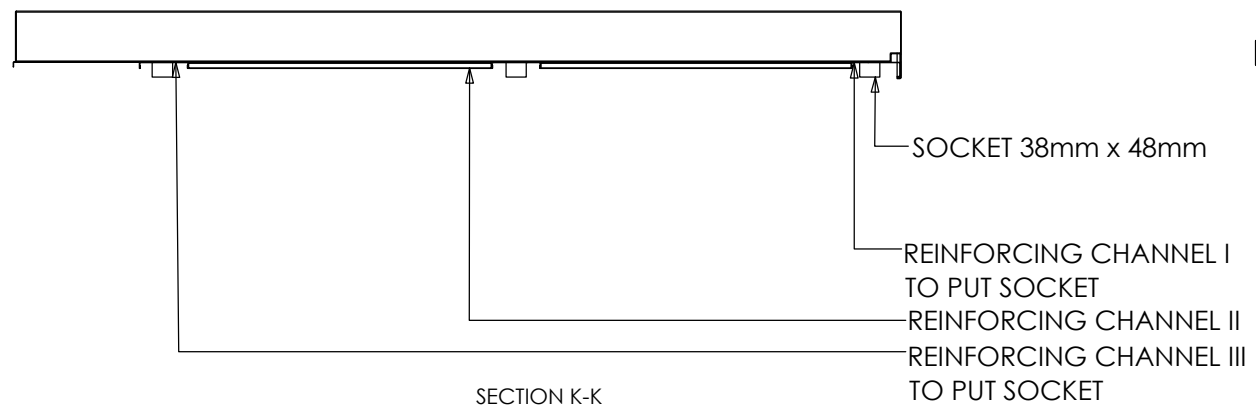
SECTION K-K
