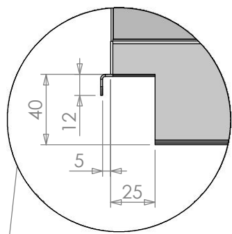
NOTCH DETAIL
