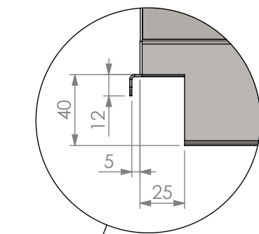
NOTCH DETAIL
