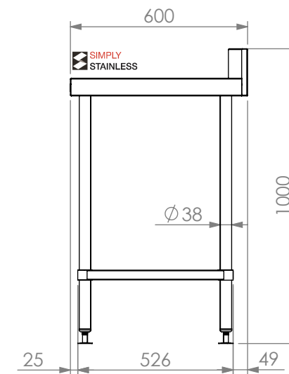
SIDE ELEVATION
