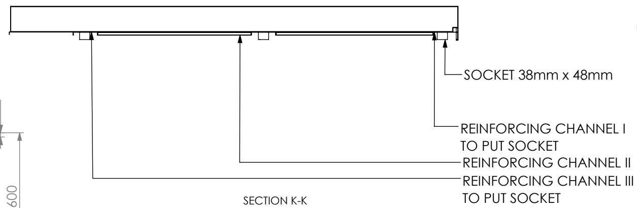
SECTION K-K
