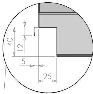
NOTCH DETAIL
