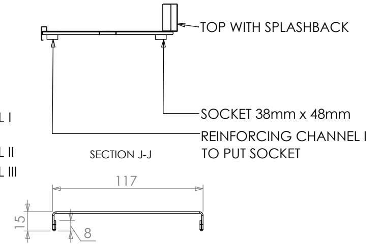
REINFORCING CHANNEL I DETAIL
