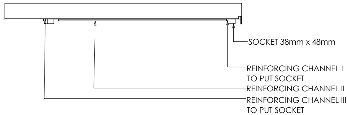
SECTION K-K
