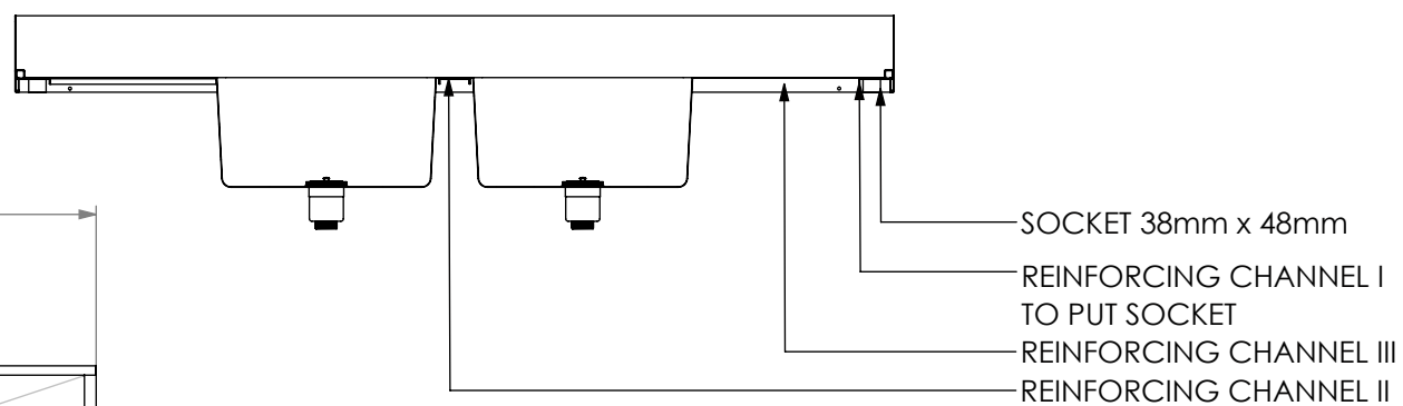
SECTION K-K
