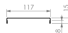
REINFORCING CHANNEL III DETAIL
