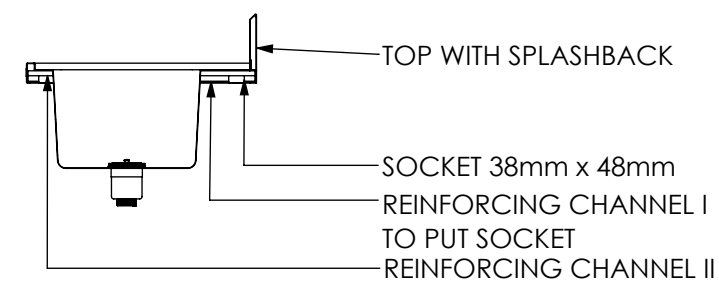
SECTION J-J
