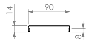
REINFORCING CHANNEL II DETAIL
