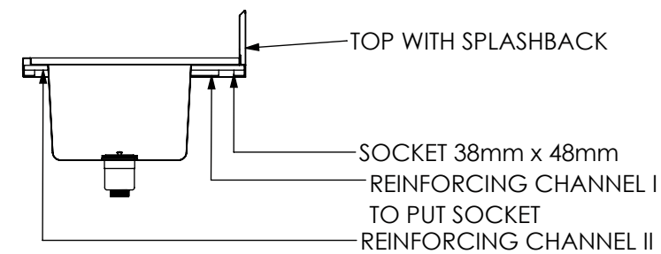
SECTION J-J
