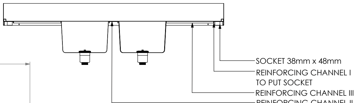
SECTION K-K
