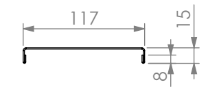
REINFORCING CHANNEL III DETAIL
