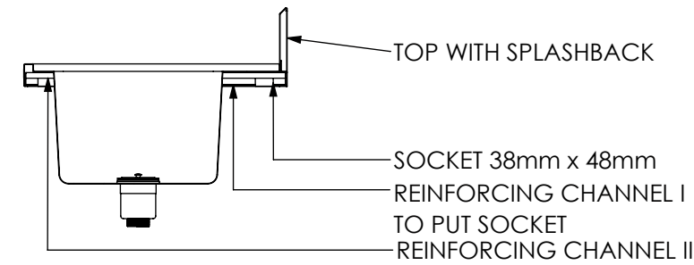
SECTION J-J
