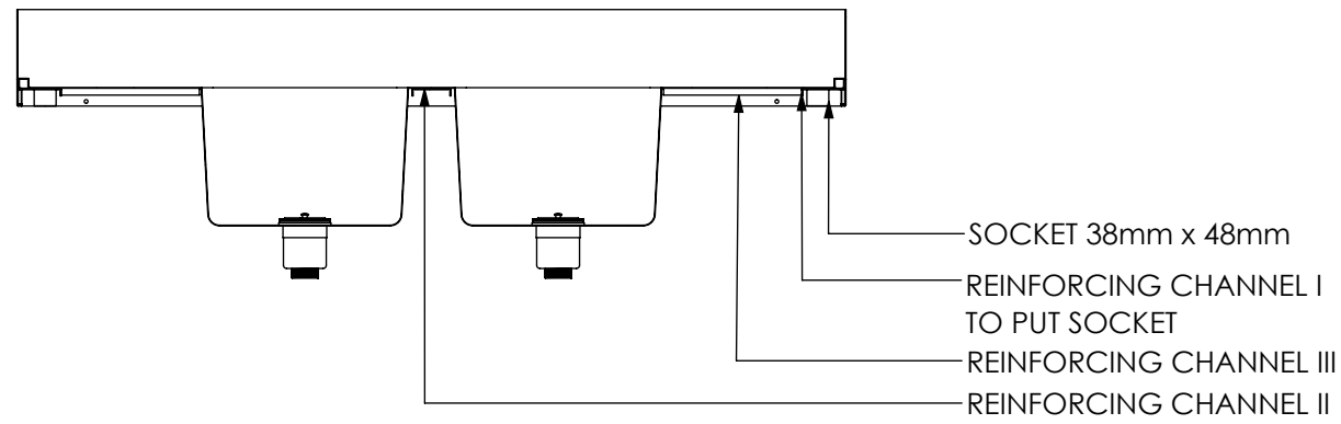
SECTION K-K
