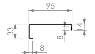
REINFORCING CHANNEL I DETAIL
