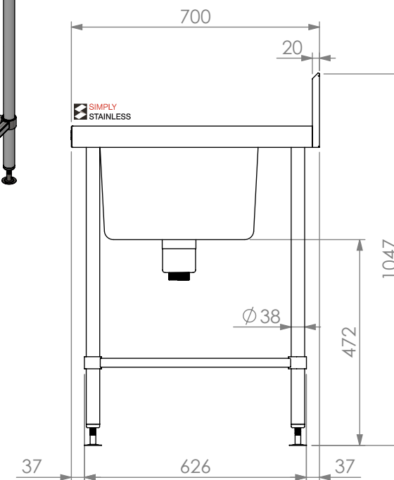
SIDE ELEVATION
