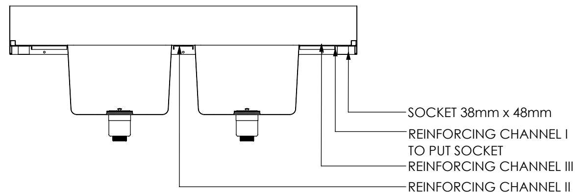
SECTION K-K
