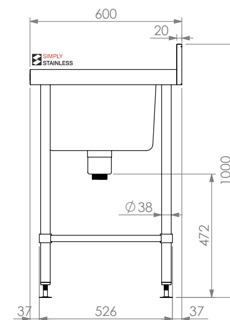
SIDE ELEVATION
