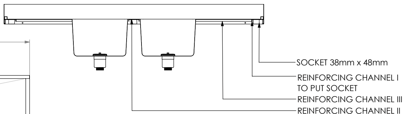
SECTION K-K
