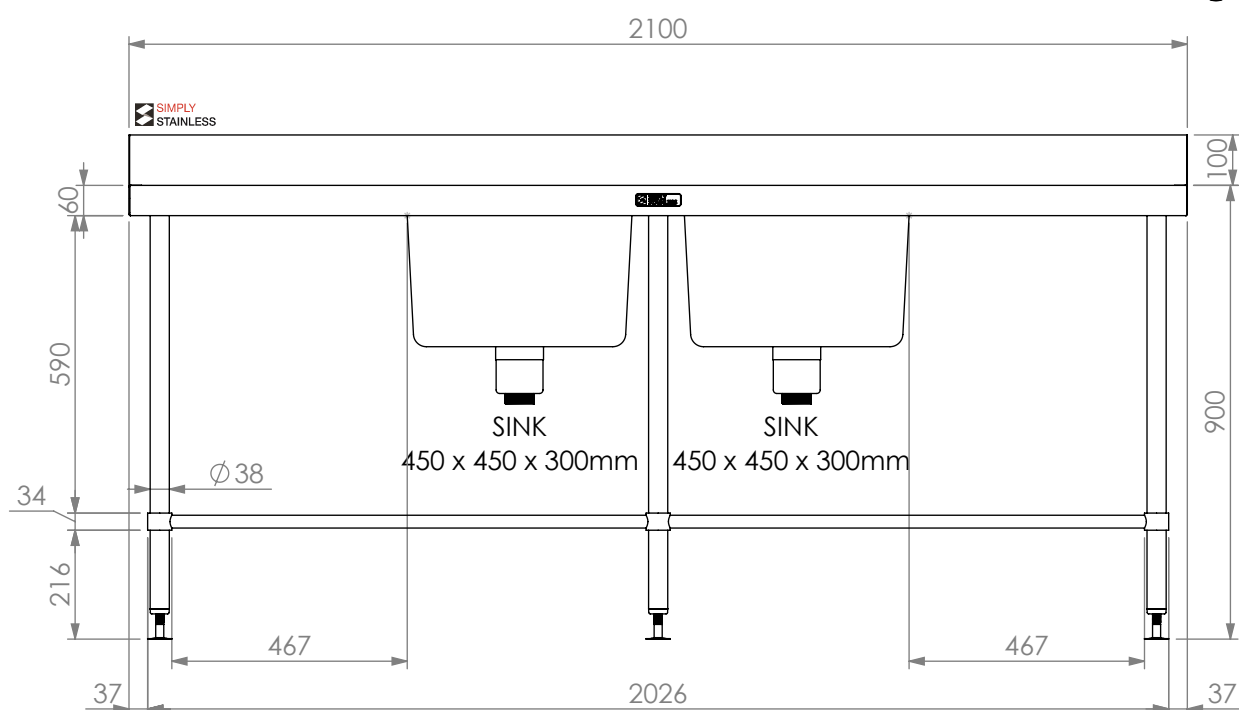
FRONT ELEVATION
