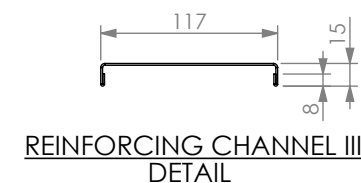
REINFORCING CHANNEL II DETAIL
