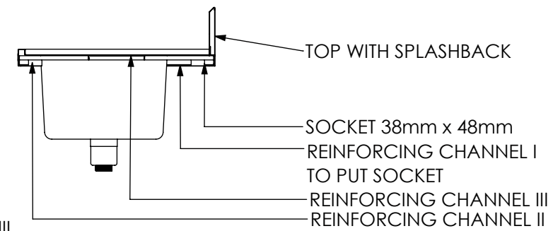
SECTION J-J
