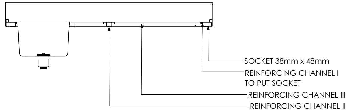
SECTION K-K
